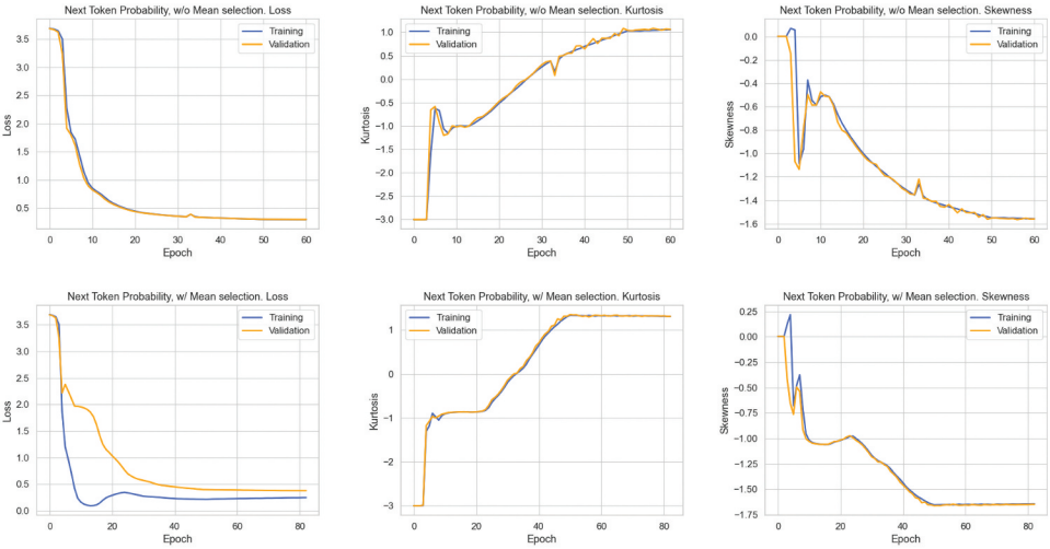
Figure A4. The evolution of the autoregressive language model next token probability distribution. HDF5 dataset.
