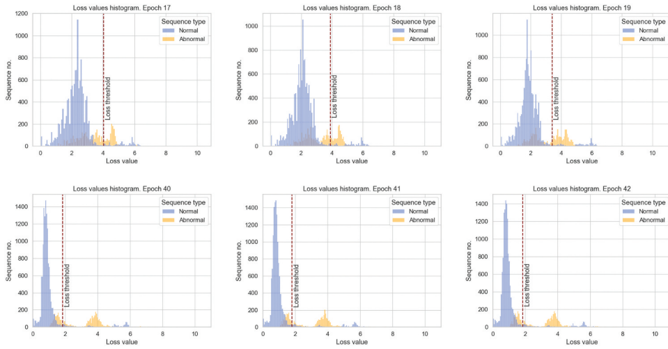
Figure A2. The evolution of the loss threshold. HDFS dataset.
