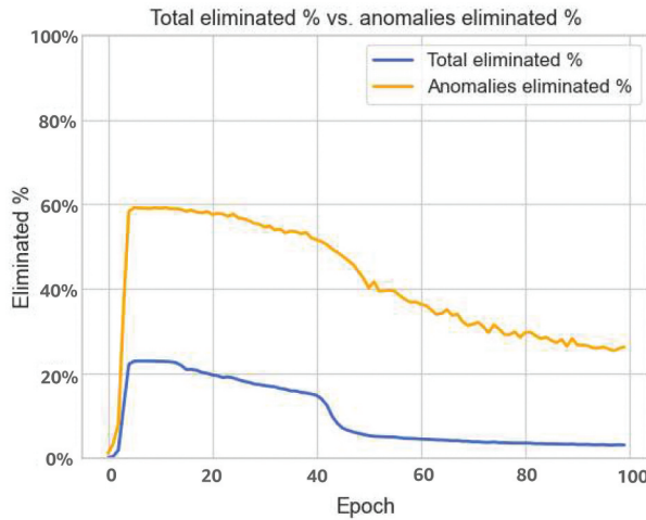
Figure 4. The percentage of eliminated sequences per epoch on the HDF5 dataset.
