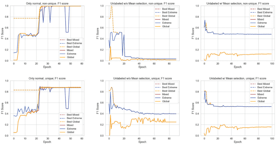
Figure 7. F1 scores for non-unique testing data (first row) and unique testing data (second row); BGL dataset, session grouping strategy.
