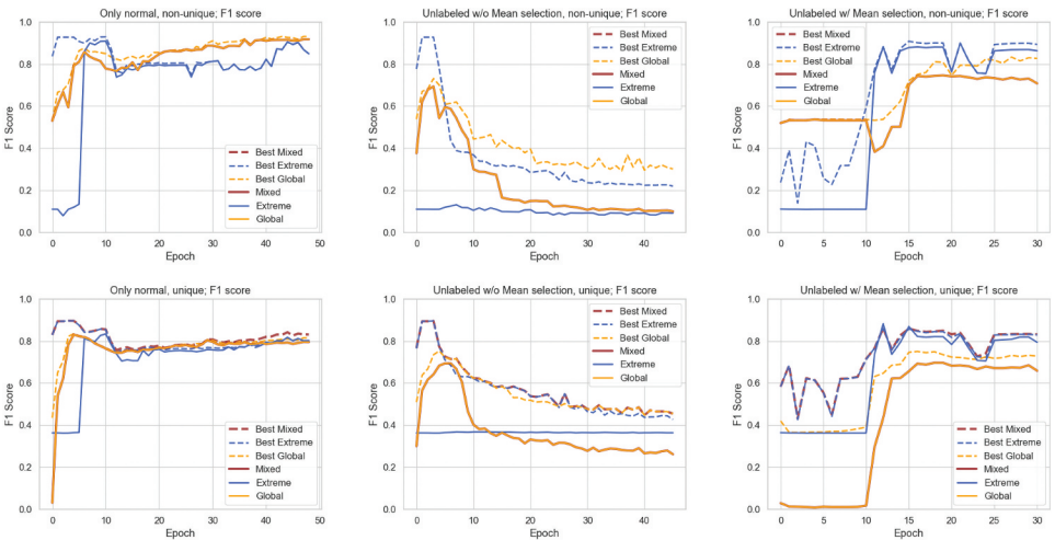
Figure 5. F1 scores for non-unique testing data (first row) and unique testing data (second row); HDFS dataset.
