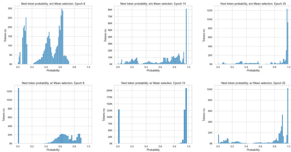
Figure A3. The evolution of the autoregressive language model next token probability. HDFS dataset.
