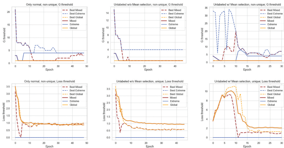
Figure 6. The evolution of the g hyperparameter and loss threshold; HDFS dataset.
