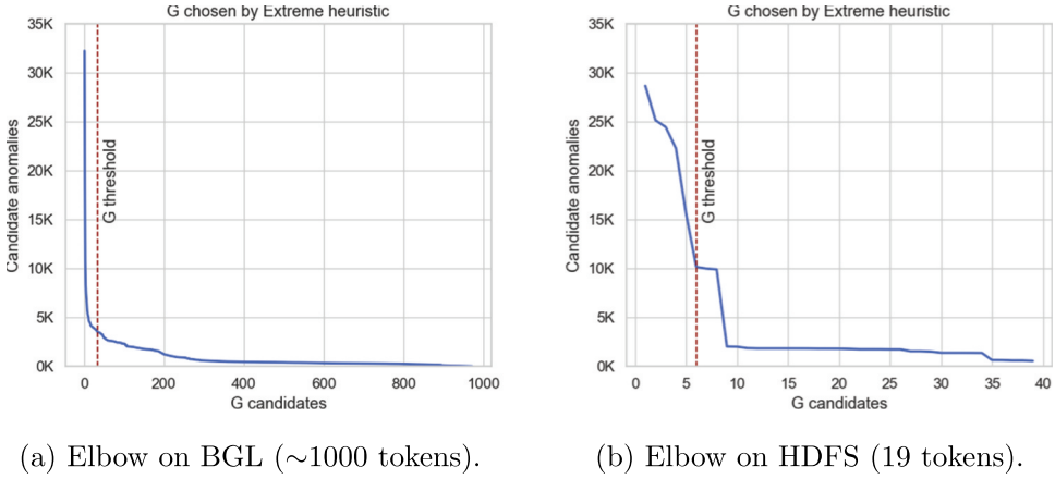
Figure 1. Anomalies curves for different values of hyperparameter g .
