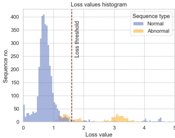
Figure 3. Histogram of testing sequences' loss values.
