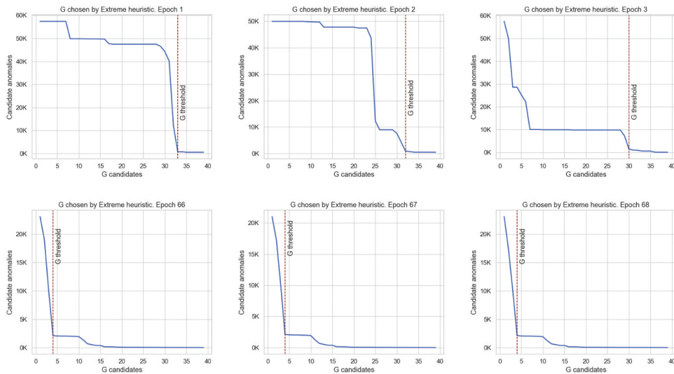
Figure A1. The evolution of the G threshold. HDFS dataset.
